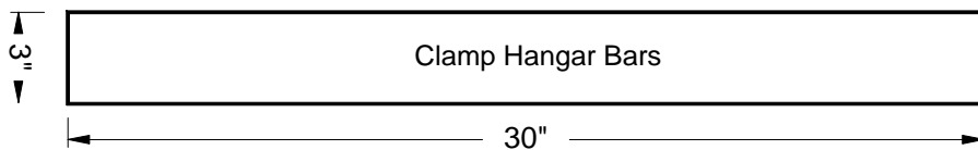
Clamp Hangar Bars 1X3" Material 4 Needed
